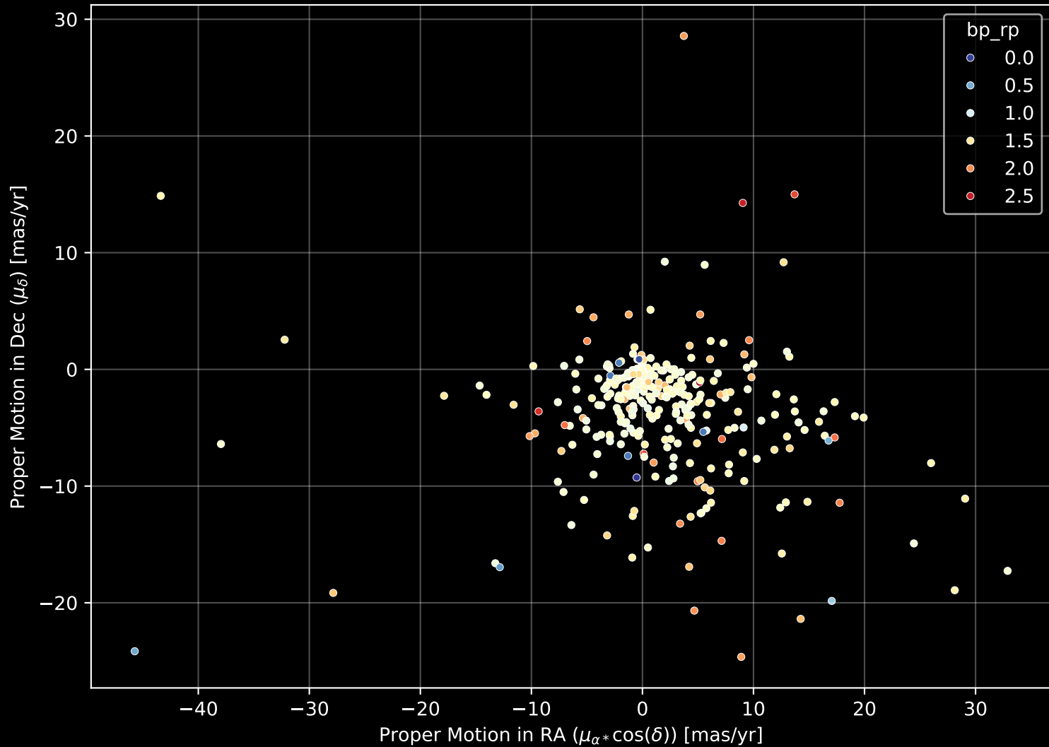
APOGEE DR17 Field: [140-24_btx] Proper Motion Diagram (n= 322)
