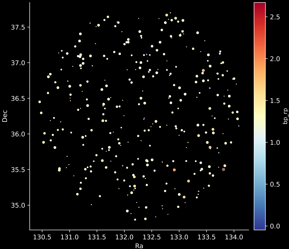
APOGEE DR17 Field: [140-24_btx] Stars: 322
