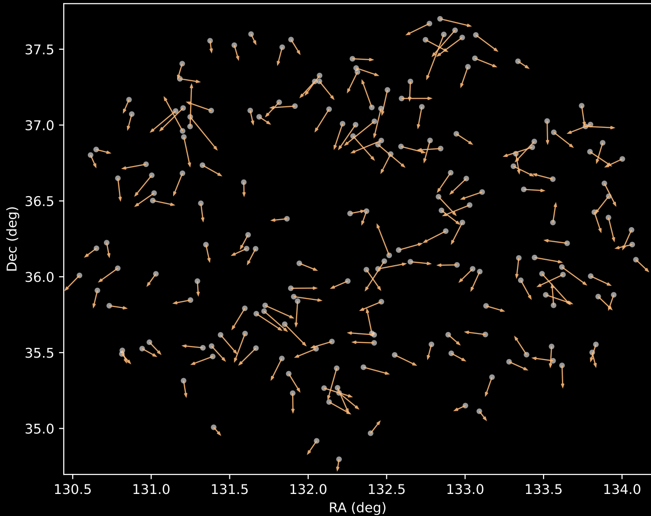
APOGEE DR17 Cluster 3 Proper Motion Vectors (n=188)
