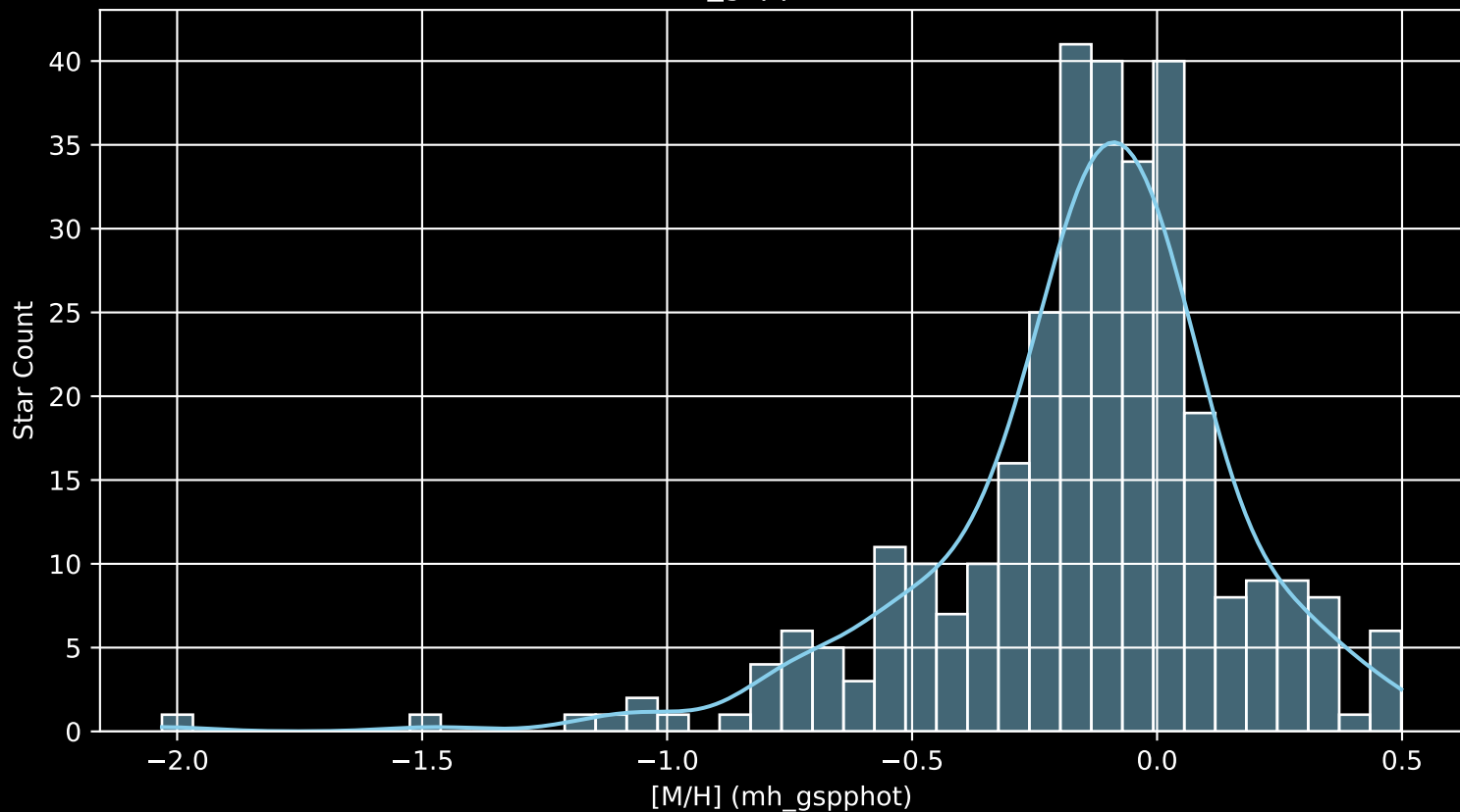
APOGEE DR17 Field: [140-24_btx [M/H] (mh_gspphot) (n= 320)
