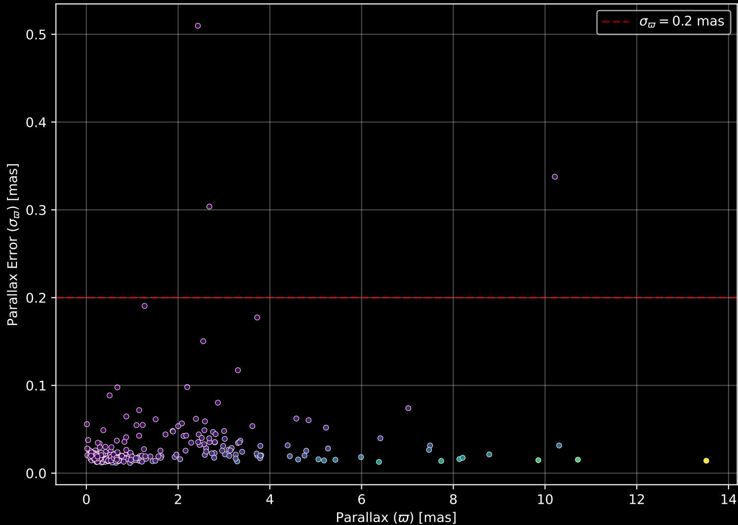
APOGEE DR17 Field: [140-24_btx] Parallax Quality (n= 322)
