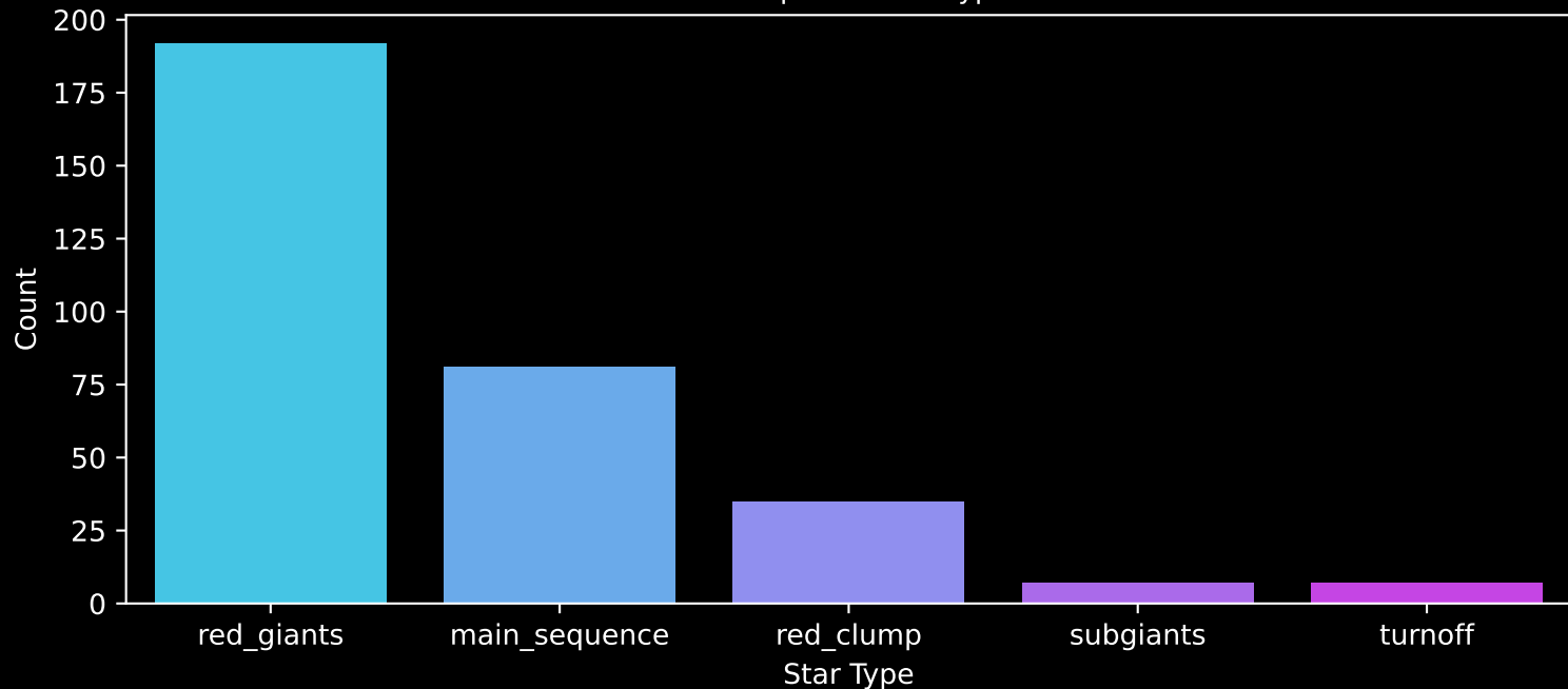
APOGEE DR17 Field: [140-24_btx] Count plot of Star Type
