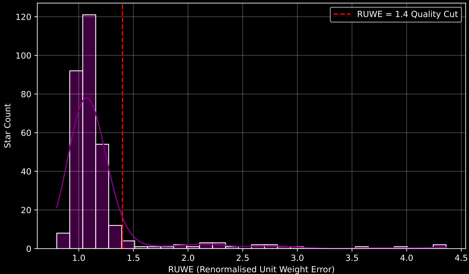
GAPOGEE DR17 Field [140-24_btx] RUWE Distribution (n= 314)
